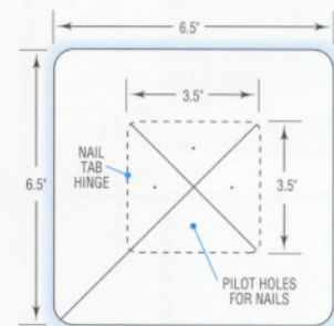
Dri-Seal 44
