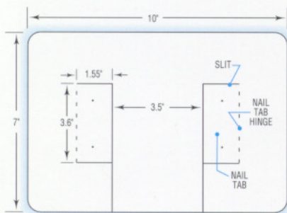
Dri-Seal 24
