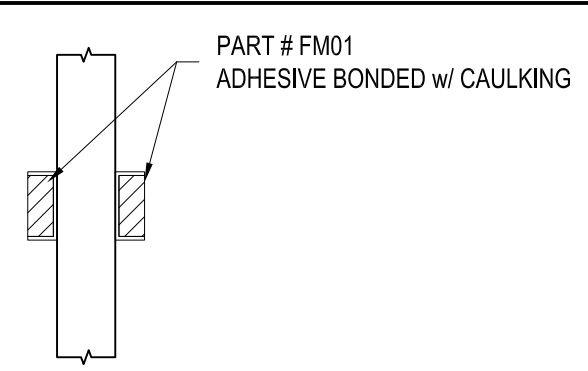
FOAM SEALER INSTALLATION DETAIL
