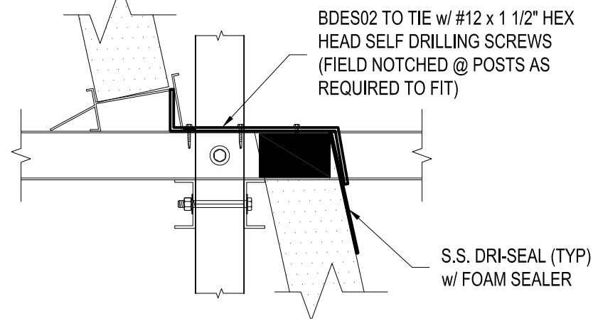
DETAIL C
