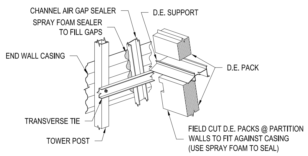
DRIFT ELIMINATOR INSTALLTION DETAIL
