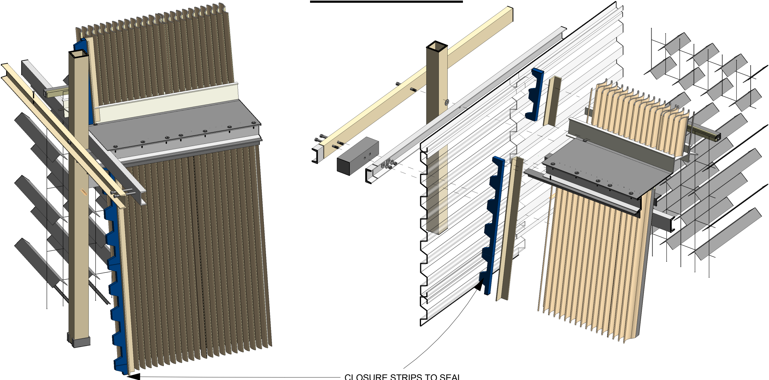
CLOSURE STRIPS TO SEAL 120Z 4.2 PANELS TO XF150MAX DRIFT ELIMINATORS
