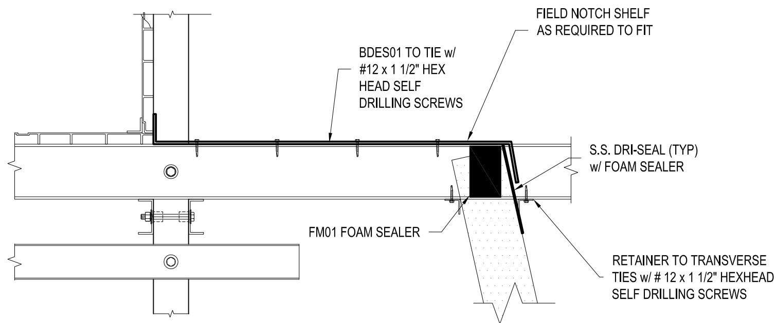
DETAIL A
