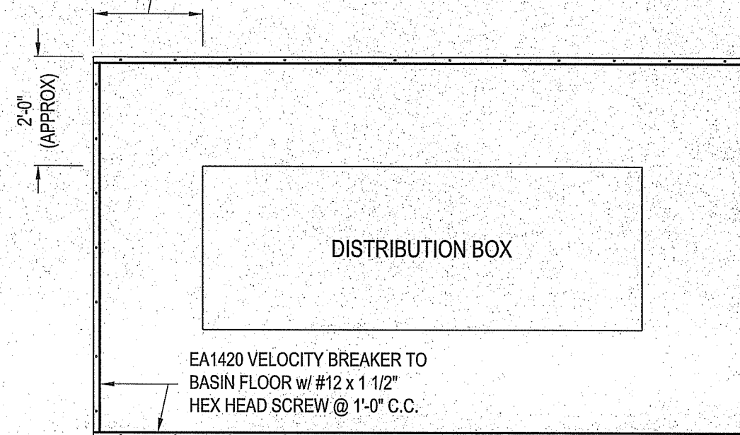
PLAN VIEW VELOCITY BREAKER INSTALLATION (TYP)
