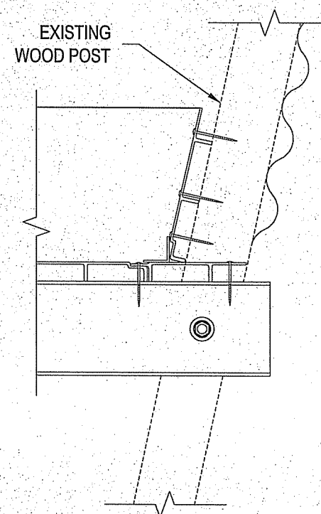
DETAIL B
