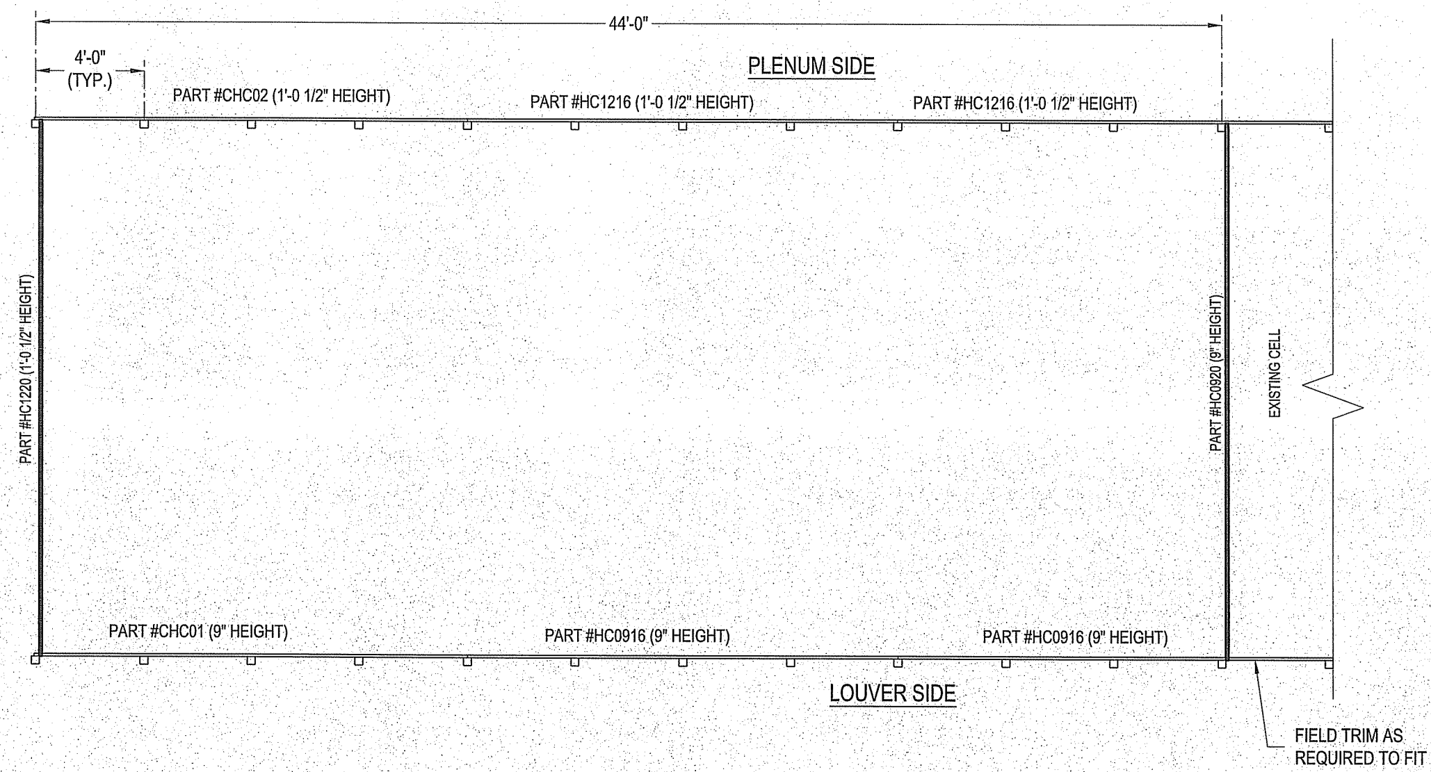
PLAN VIEW (CURB LAYOUT)
