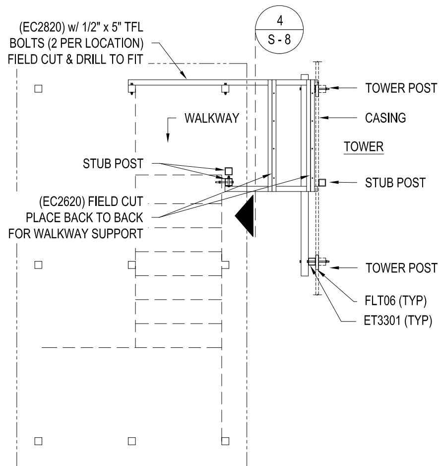
DETAIL A PLAN VIEW SECTION TOP TIEBACK INSTALLATION
