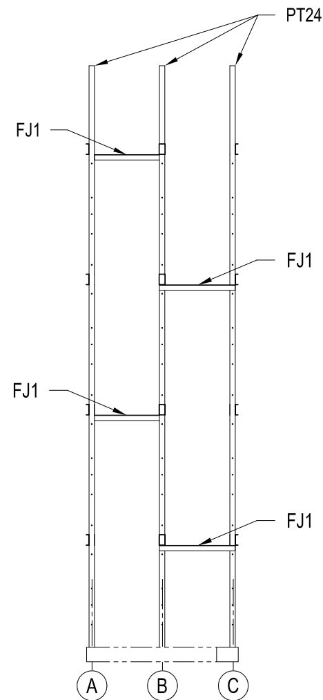
STAIR POST ROW 3
