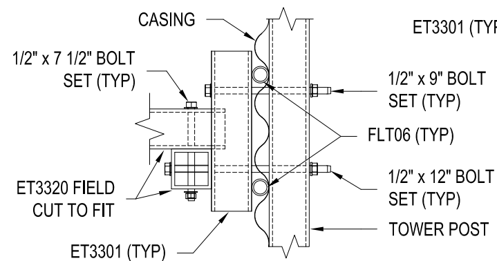
SIDE VIEW MID TIE BACK
