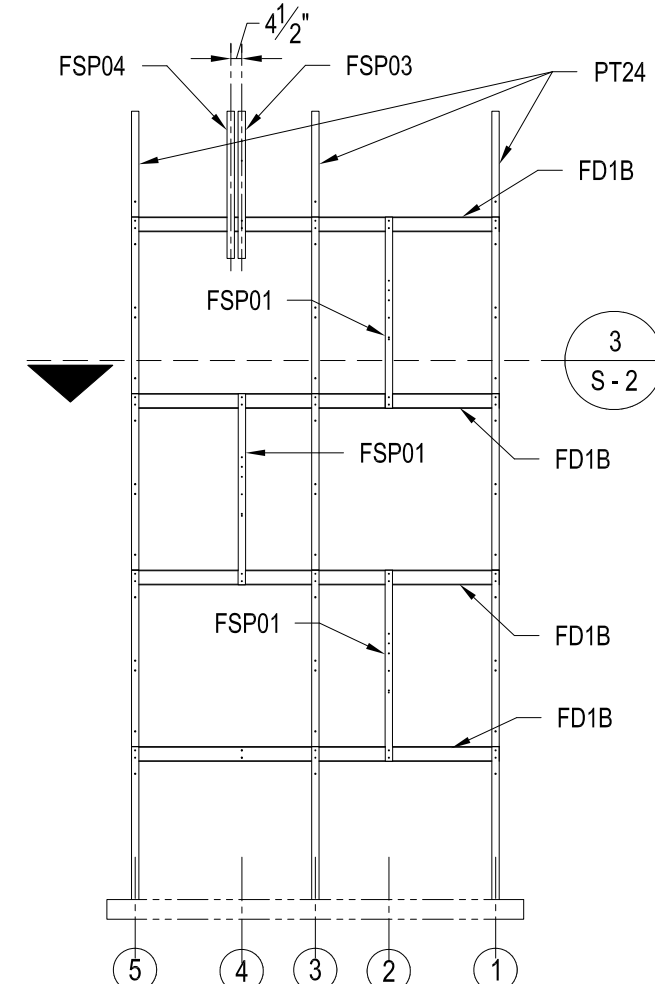
STAIR POST ROW C
