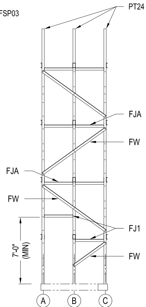
STAIR POST ROW 5
