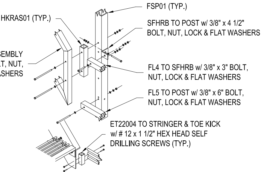
DETAIL D HAND, KNEE RAIL ASSEMBLY @ POST END PLATFORM UP STRINGER
