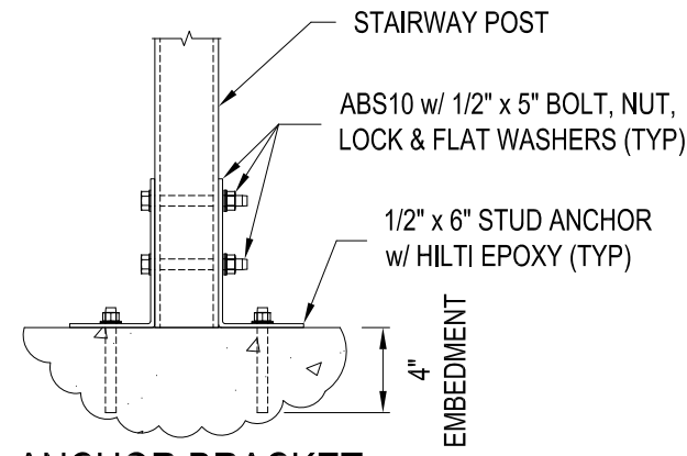
ANCHOR BRACKET INSTALLATION
