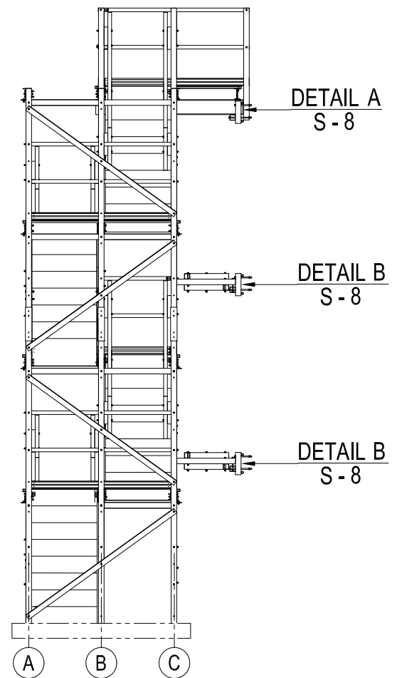
STAIR ASSEMBLY w / TIE BACK
