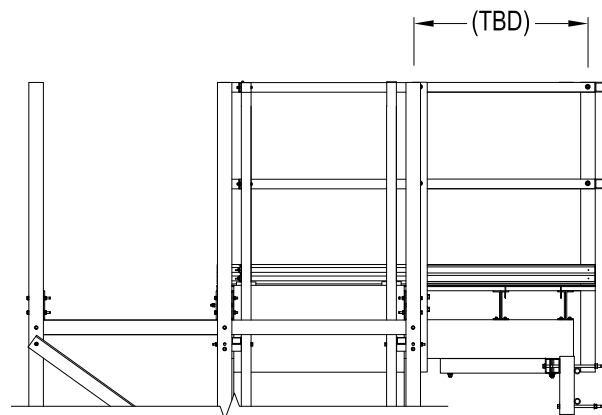
SIDE VIEW TOP TIE BACK INSTALLATION
