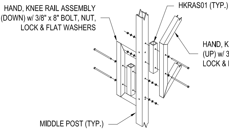
DETAIL C HAND KNEE RAIL ASSEMBLY@ POST MIDDLE PLATFORM
