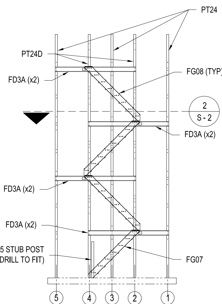
STAIR POST ROW B
