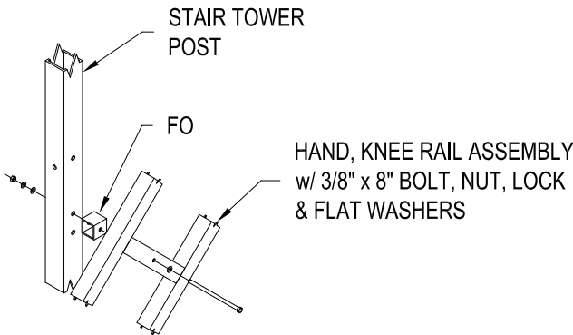
DETAIL F HAND, KNEE ASSEMBLY @ MIDDLE STRINGER & POST
