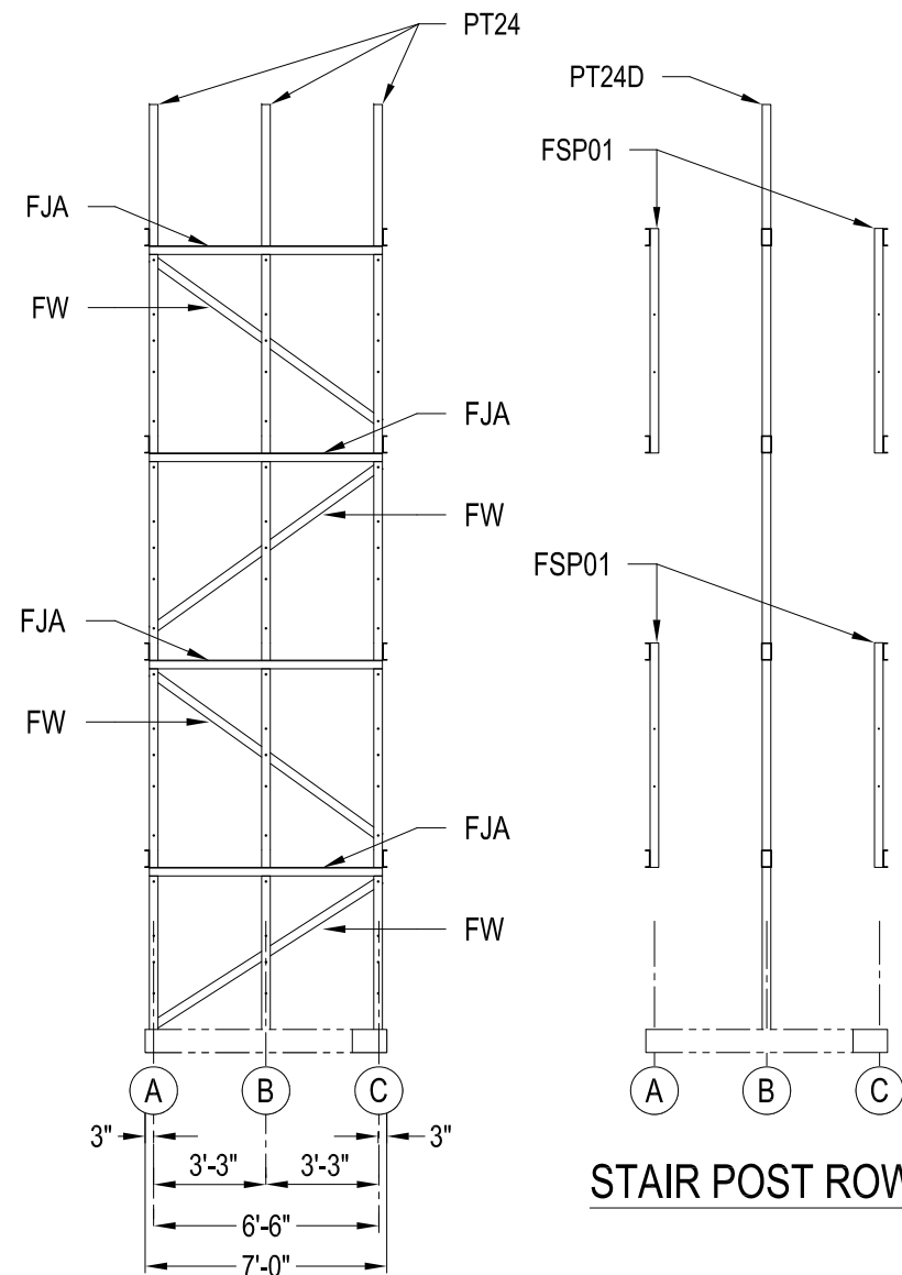
STAIR POST ROW 1
