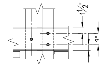
DETAIL A1 FIELD DRILL PATTERN
