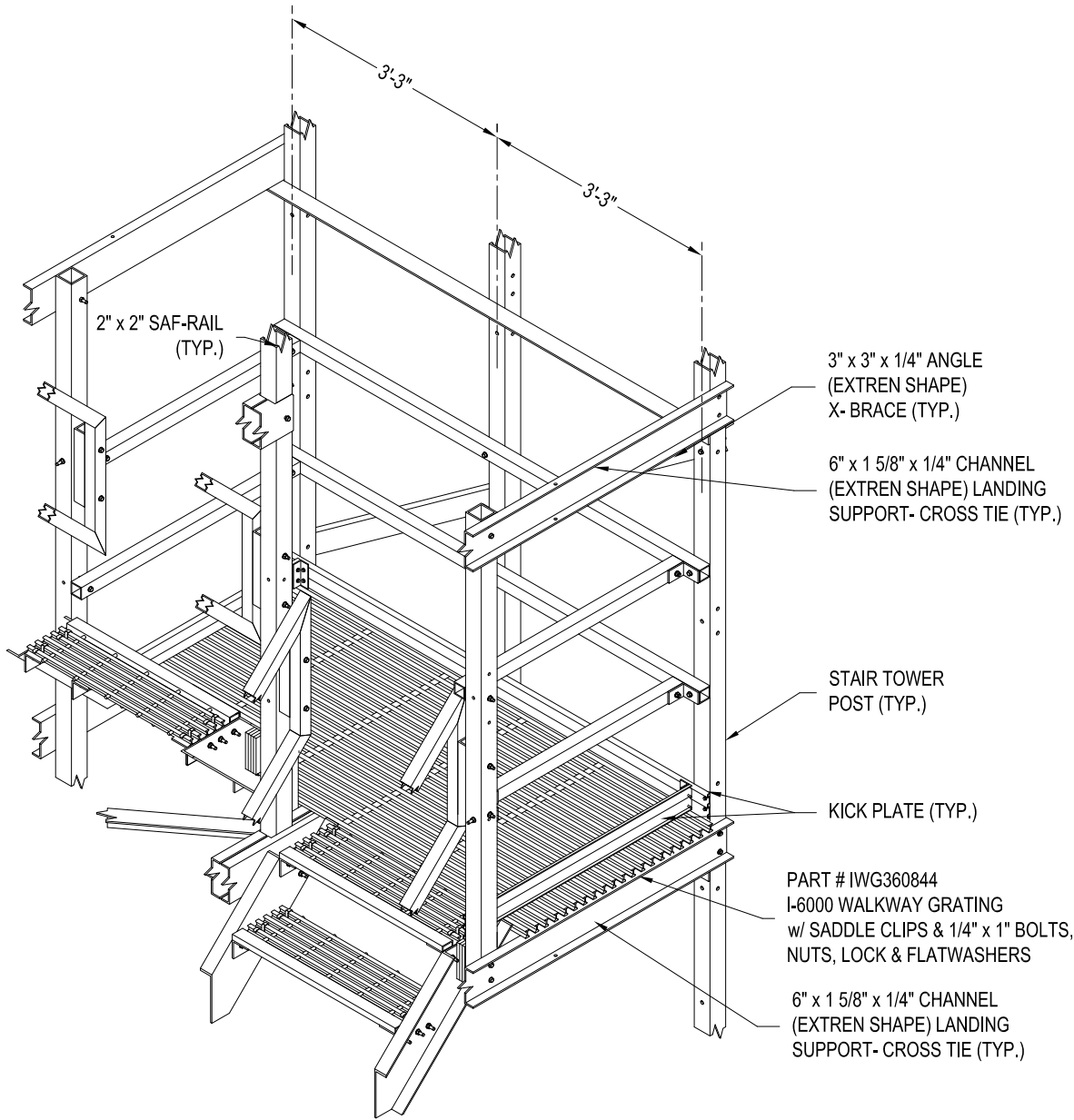
STAIRWAY LANDING INSTALLATION DETAIL (TYP.)
