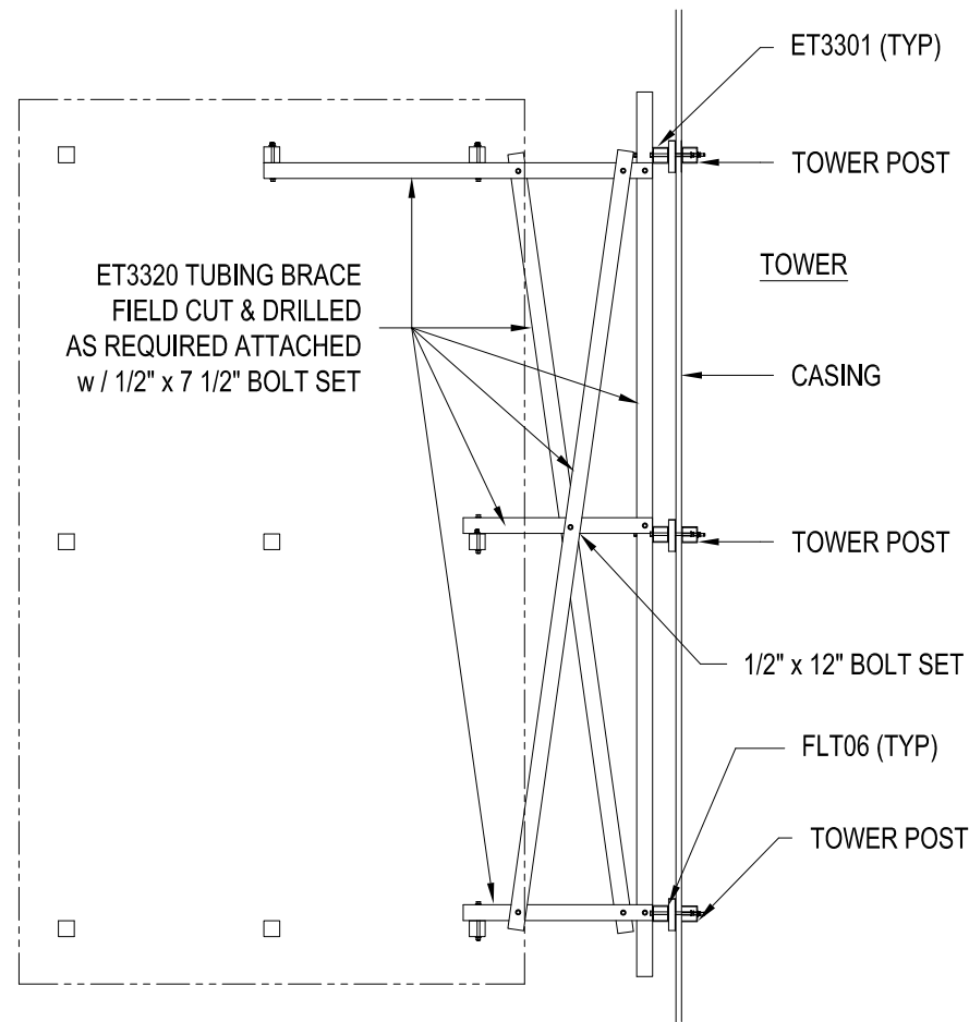
DETAIL B PLAN VIEW SECTION INTERMEDIATE TIEBACK INSTALLATION
