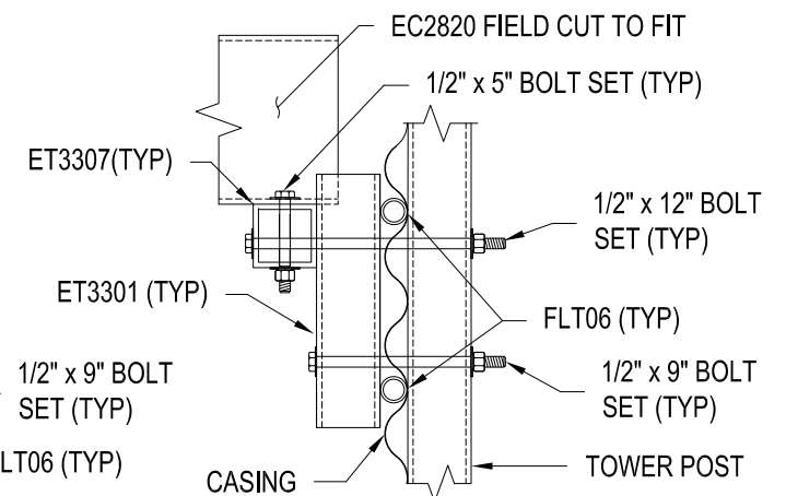
SIDE VIEW TOP TIE BACK
