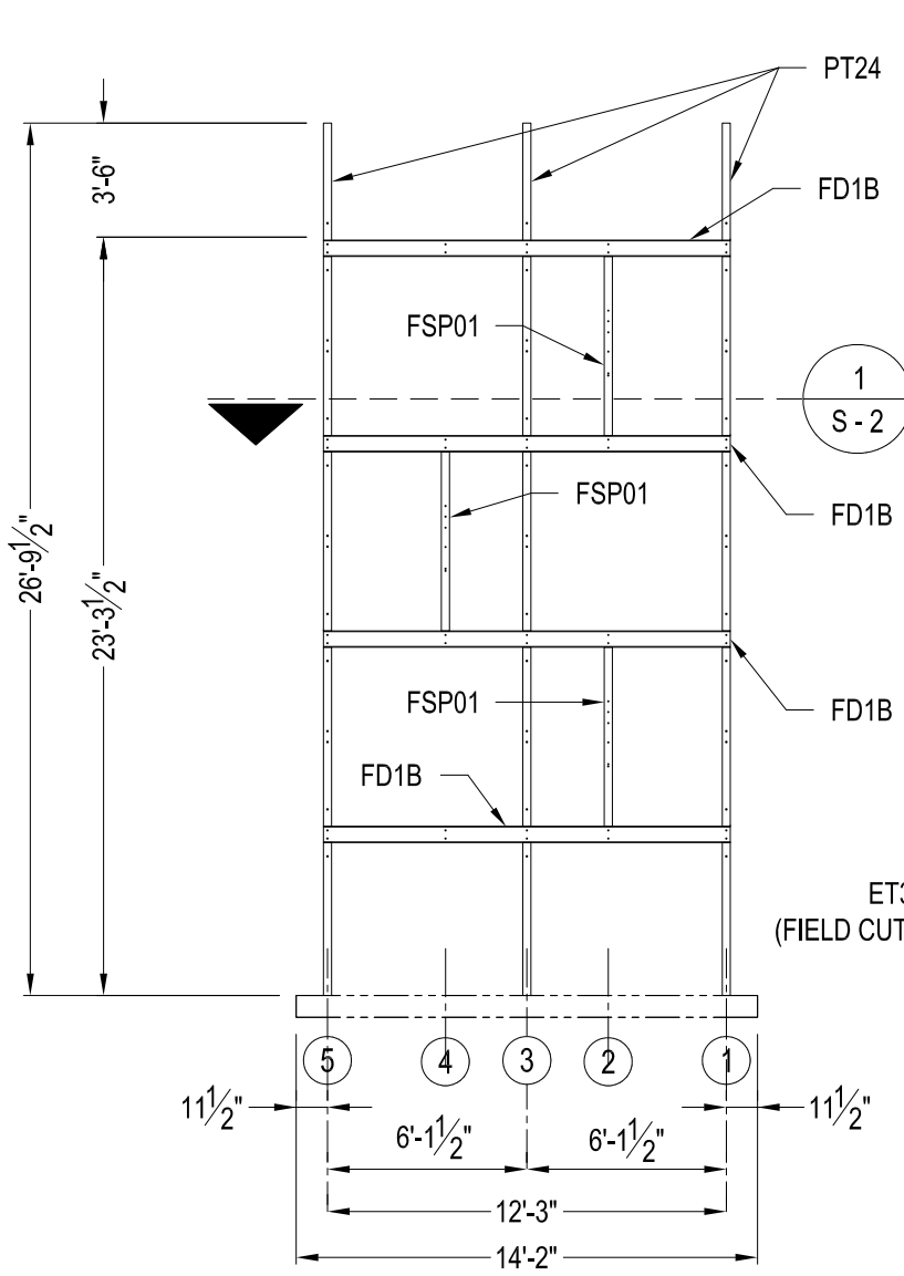
STAIR POST ROW A
